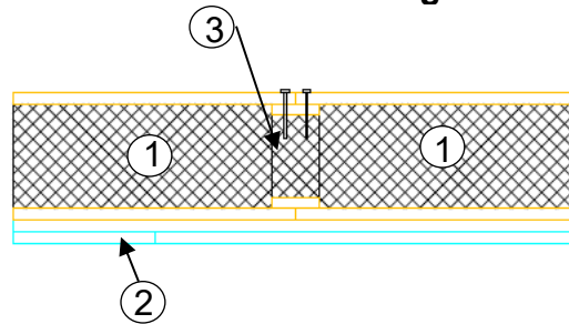
Vertical Section
