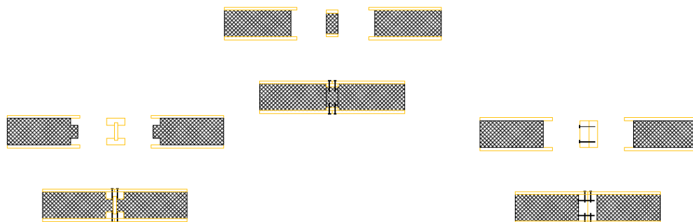
FIGURE 1—PREMIER SIP SPLINE TYPES
